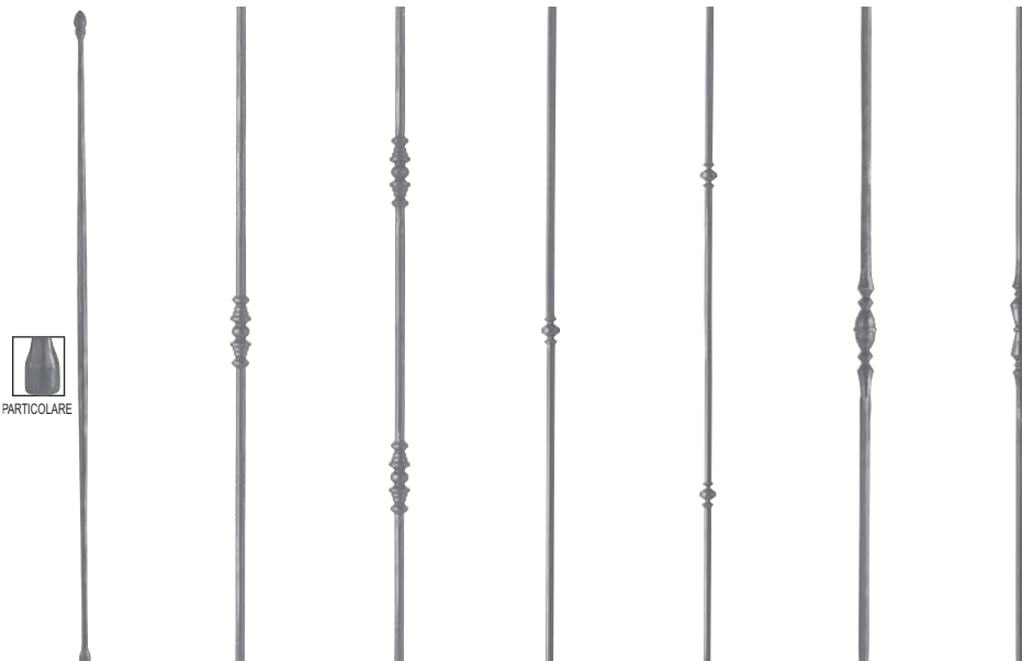
H.1000 mm. Art. 11.041.33 Ø 14 circa H.1000 mm. Art. 11.041.34 Ø 14 mm H.1000 mm. Art. 11.041.35 Ø 14 mm H.1000 mm. Art. 11.041.36 Ø 12 mm H.1000 mm. Art. 11.041.37 Ø 12 mm H.1000 mm. Art. 11.041.38 □ 14 circa H.1000 mm. Art. 11.041.39 Ø 12 mm
