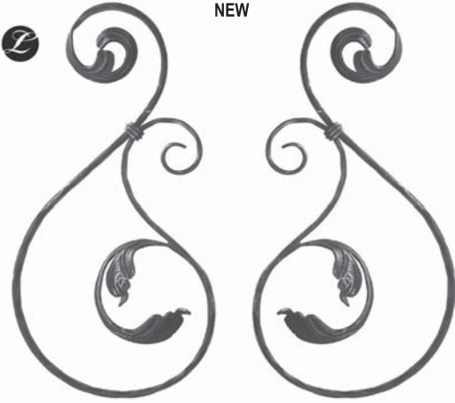
Martellato / Hammered H.500 x L.260 mm Art. 04.408 \neq 16 x 8 mm Sinistro / Left
